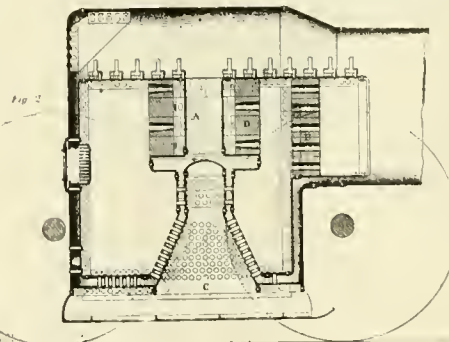
YATES FIRE BOX. FIG. 73. Used on Buffalo & Lake Huron Railway.
